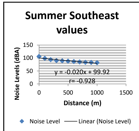
Fig.1: Summer southeast graphical presentation of noise results
