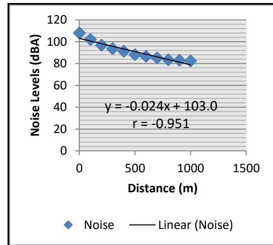
Fig. 3– Winter southeast graphical presentation of noise level
