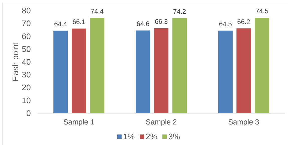
Figure 2: Flash point at different biodiesel percentage
