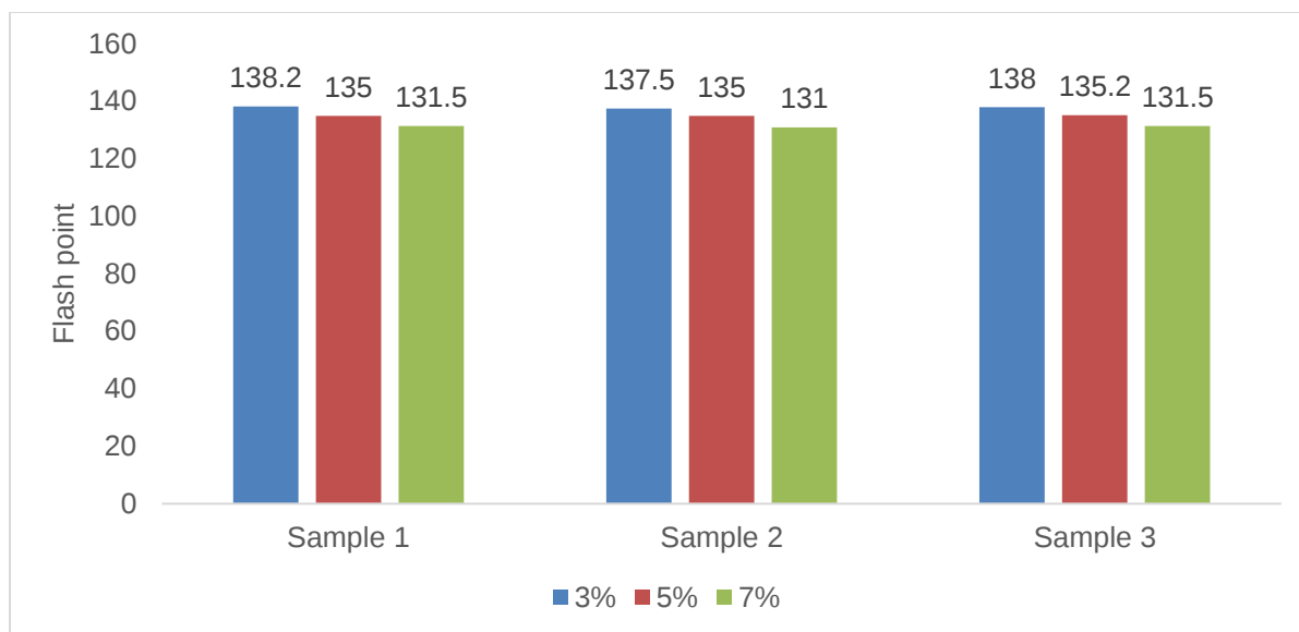
Figure 1: Flash point at different percentage interface
