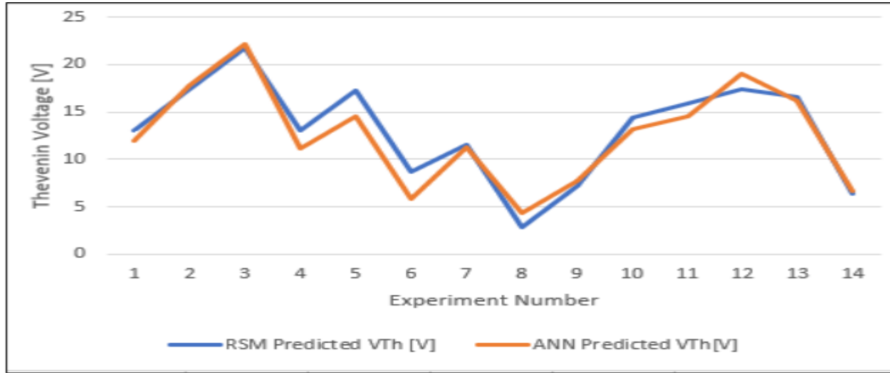
Figure 2: Variation of V_{TH} values
