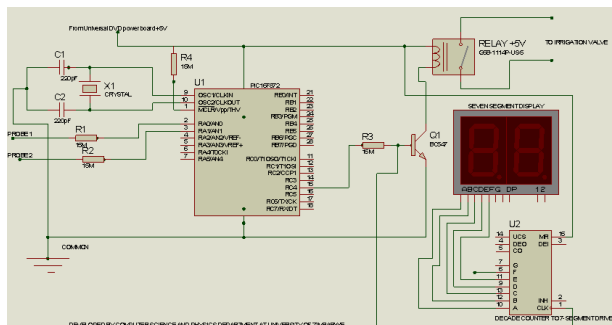
Figure 1: Soil moisture-based irrigation controller circuit diagram
