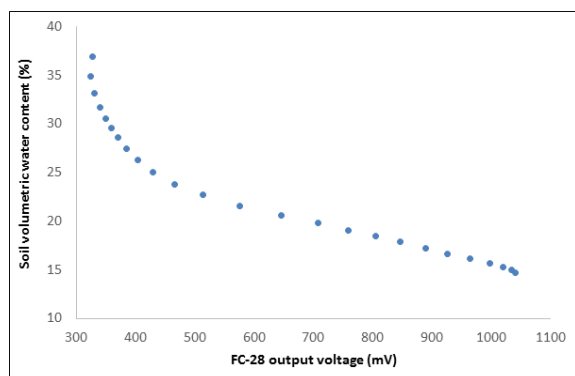
Figure 3: Relationship between the output voltage and the soil moisture for the FC-28 dielectric soil moisture sensor
