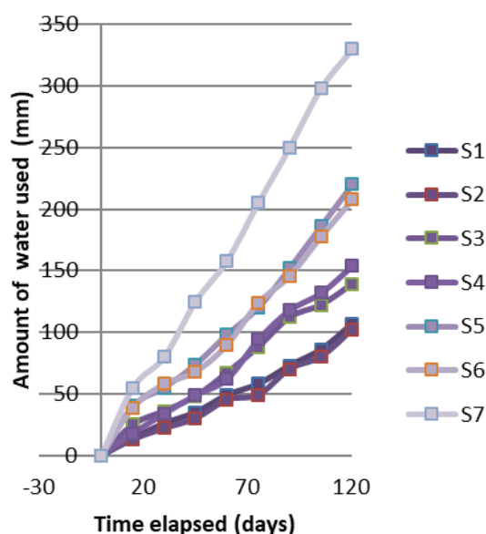
Figure 5. A plot of irrigation amount for each treatment versus the period under irrigation
