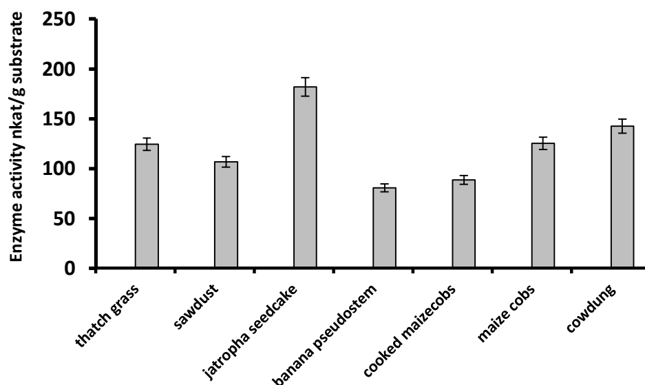
Figure 1. Cellulase production by D. phacea cultured on different cellulosic substrates over 144 hours at 25°C.
