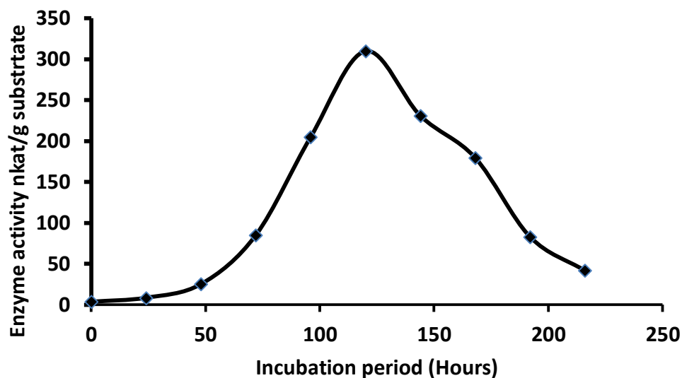
Figure 2. Time course analysis for cellulase production by D. phacea during solid state fermentation of Jatropha seed cake at 25 °C over a period of 216 hours
