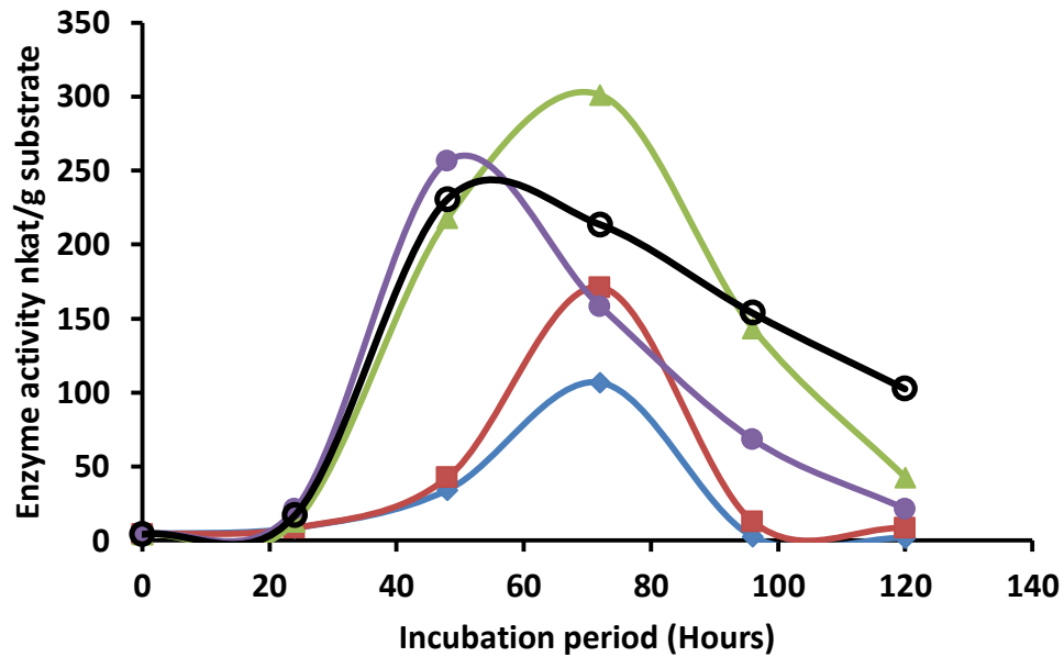
Figure 4. Effect of pH on cellulase production by D. phacea during solid state fermentation of Jatropha seed cake at pH 4 (♦), pH 5 (■), pH 6 (▲), pH 7 (●) and pH 8 (○) at 30 °C over a period of 120 hours
