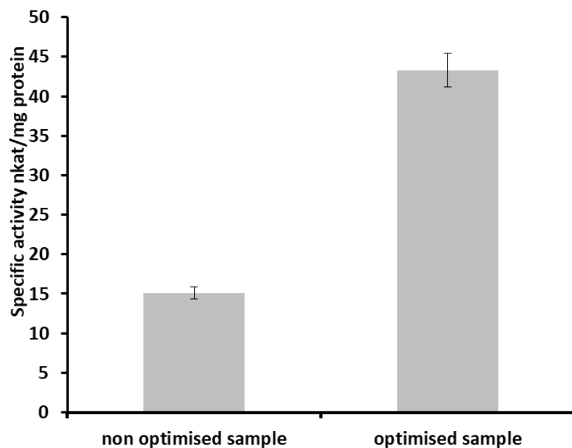
Figure 8. Effect of optimizing conditions of solid state fermentation of Jatropha seed cake on cellulase production by D. phacea
