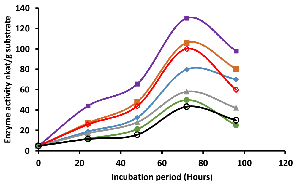
Figure 7. Effect of an additional carbon source on cellulase production by D. phacea during solid state fermentation of Jatropha seed cake over a period of 96 hours. Jatropha and 10% saw dust (◆), Jatropha and 10% cow dung (■), Jatropha and 10% cooked maize cobs (▲), Jatropha and 10% uncooked maize cobs (◇), Jatropha and 10% thatch grass (■), Jatropha and 10% banana pseudostem (●) Jatropha only (○).
