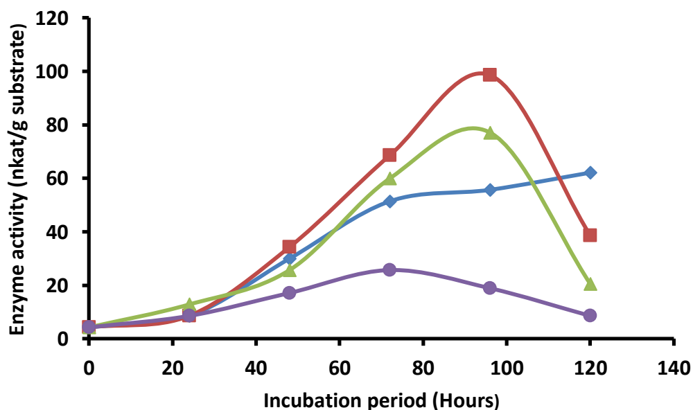
Figure 3. Effect of temperature on cellulase production by D. phacea during solid state fermentation of Jatropha seed cake at 25 °C (♦), 30 °C (■), 35 °C (▲) and 40 °C (●) over a period of 120 hours
