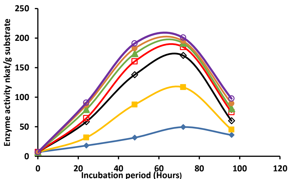
Figure 6. Effect of lactose on the production of cellulases by D. phacea during solid state fermentation of Jatropha seed cake with peptone as the nitrogen source, at 30 °C and initial pH 6 over a period of 96 hours. No lactose (♦), 0.5 g /L lactose, (■), 1.0 g/L lactose (◇), 1.5 g/L lactose (□), 2.0 g/L lactose (▲), 2.5 g /L lactose (●), 3.0 g/L lactose (○)
