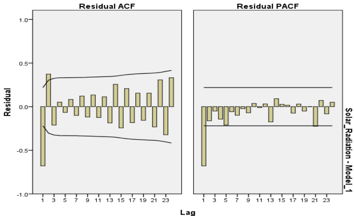
Figure 9: ACF and PCF of the time series data after differencing
