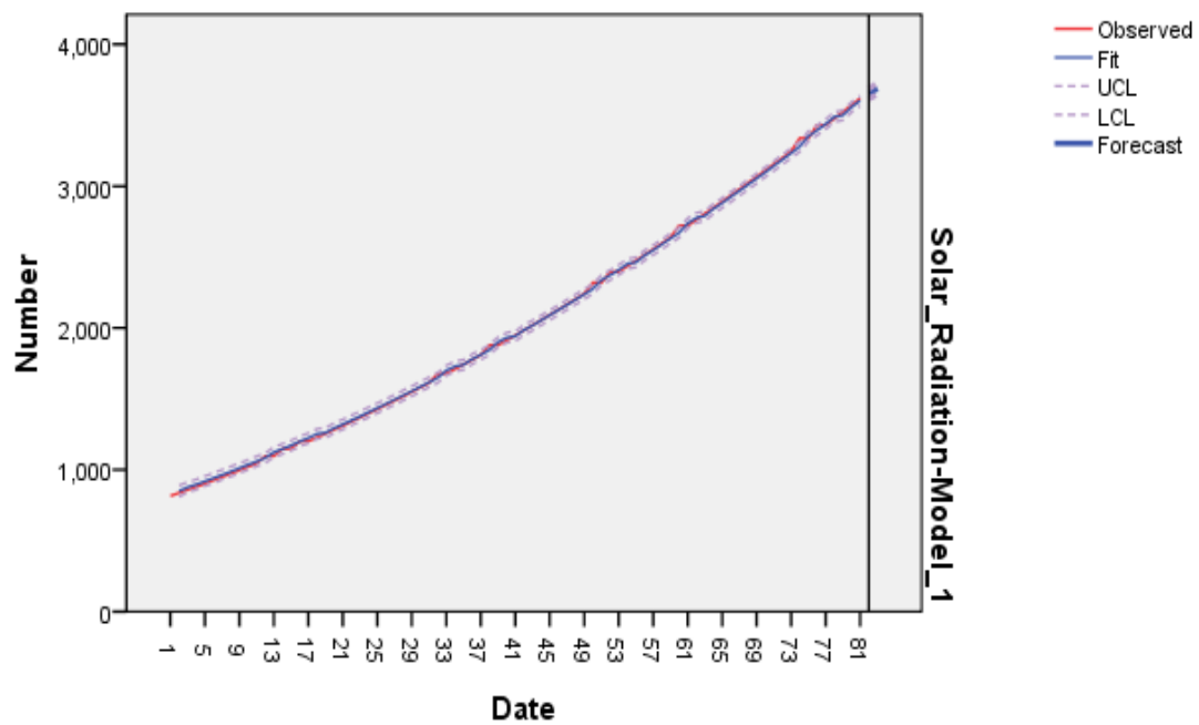
Figure 7. A forecast plot versus the actual value for the past 81 days.
