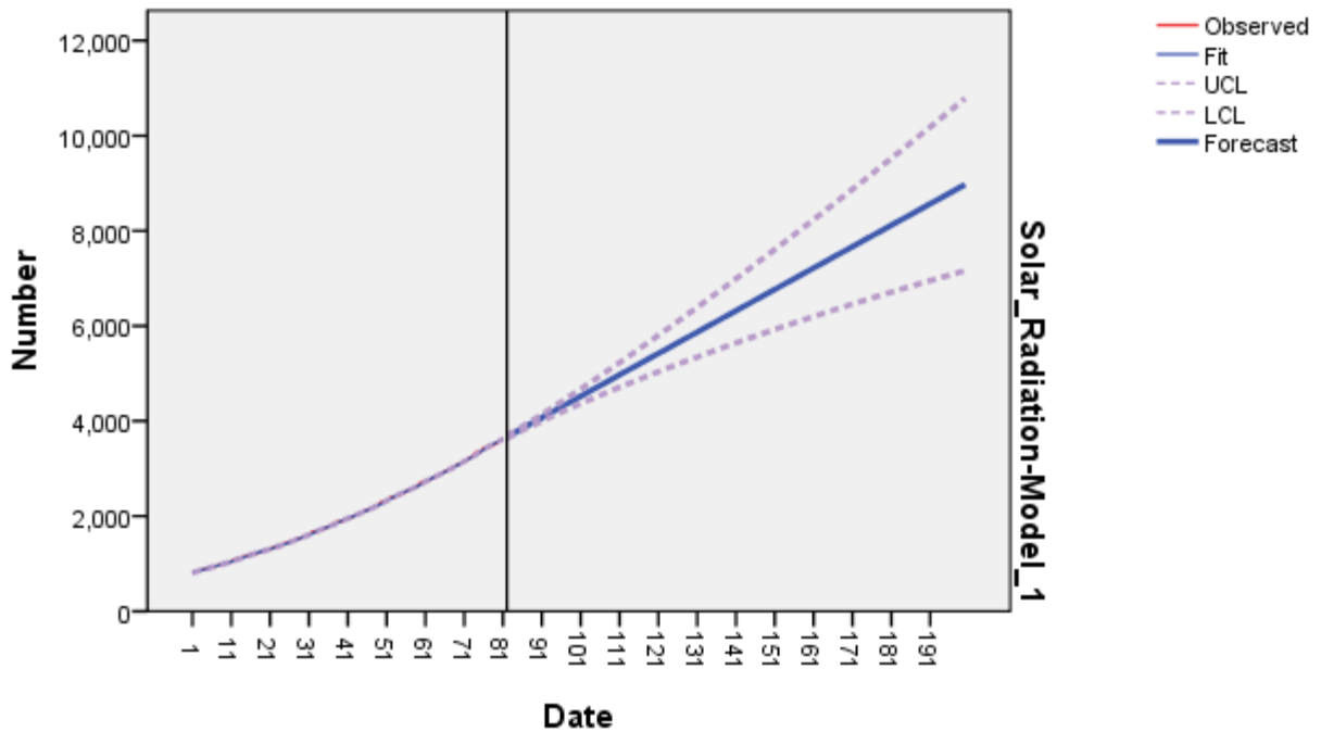
Figure 8. A clearer forecast versus actual values for the past 81days. This has shown clearly hat the UCL and LCL are drifting away from the forecast
