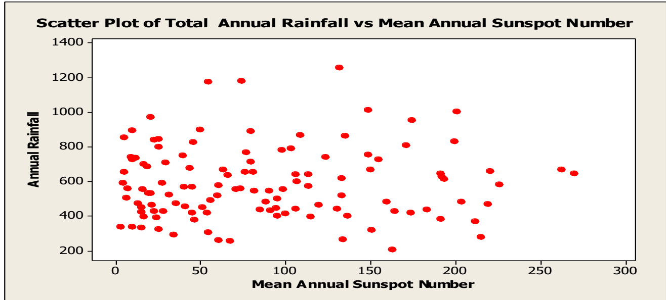
Figure 6. Scatter plot annual rainfall vs annual sunspots.
