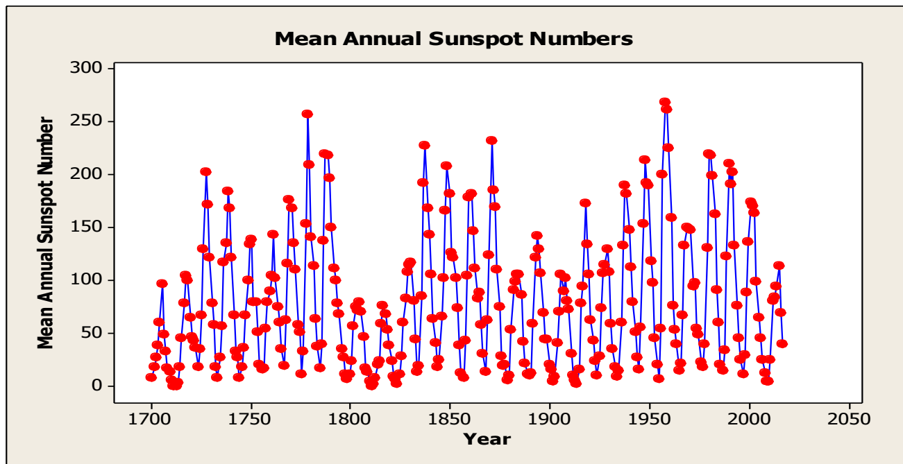
Figure 1. Time series plot of Annual Sunspot Numbers
