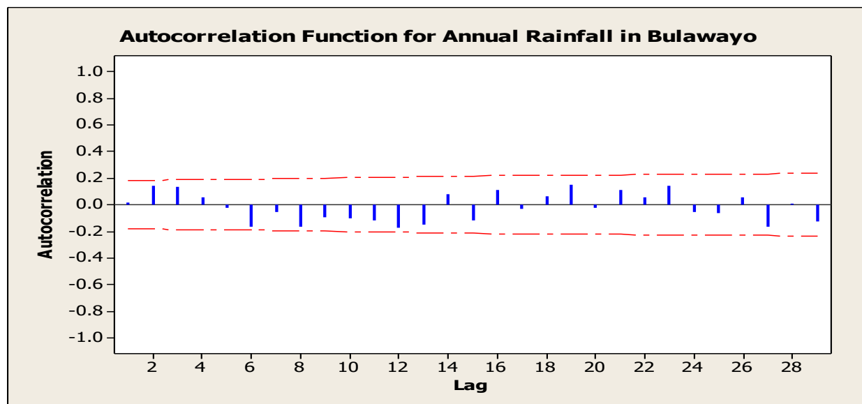
Figure 5. Autocorrelation function for Annual rainfall in Bulawayo (lag in years).
