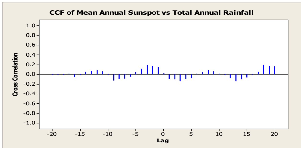
Figure 7. CCF of Mean Annual Sunspot Number and Total Annual Rainfall (lag in years).
