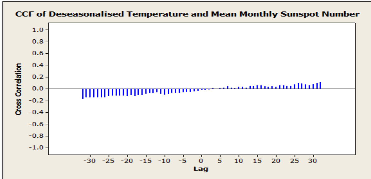
Figure 9. CCF of Mean Monthly Dry Bulb Temperature and Mean Monthly Sunspot Number (lag in months)
