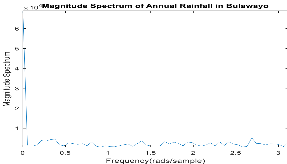
Figure 4. Periodogram of Annual Rainfall.
