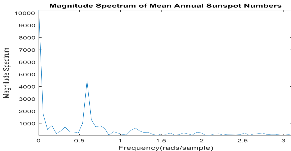
Figure 2. Mean Annual Sunspot Magnitude Spectrum.
