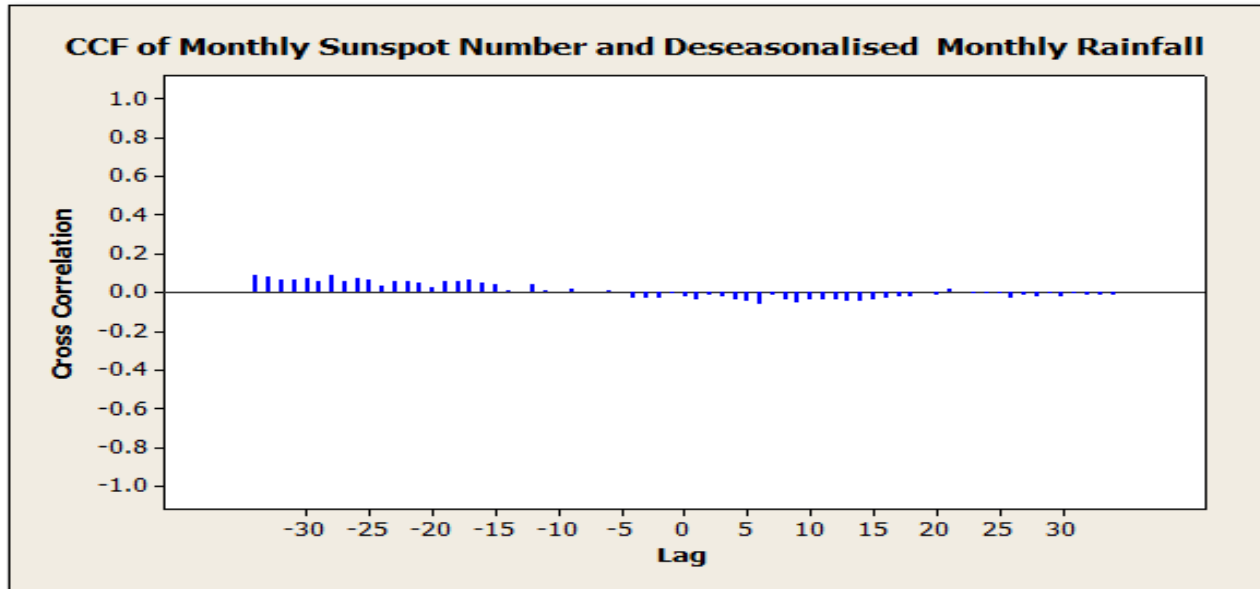
Figure 8. CCF of Mean Monthly Sunspot Number and Monthly Rainfall (lag in months).
