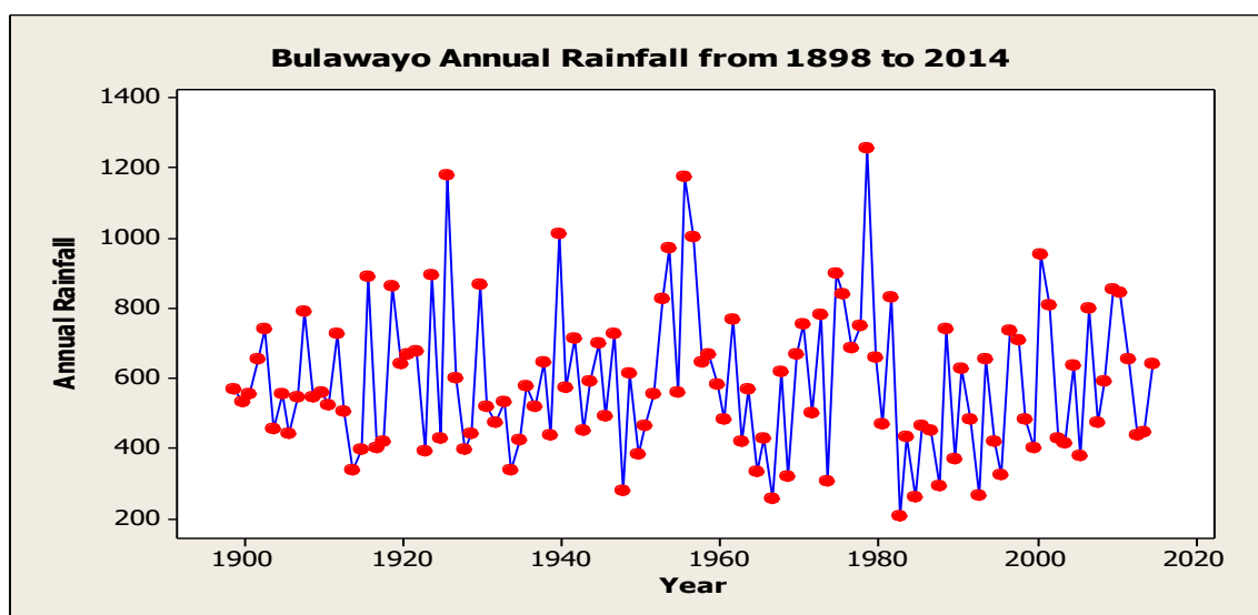
Figure 3. Time series for Bulawayo Annual Rainfall (mm)
