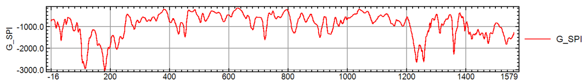
Figure 4b. Profile across Dange- Sabonbirni Sub-basin
