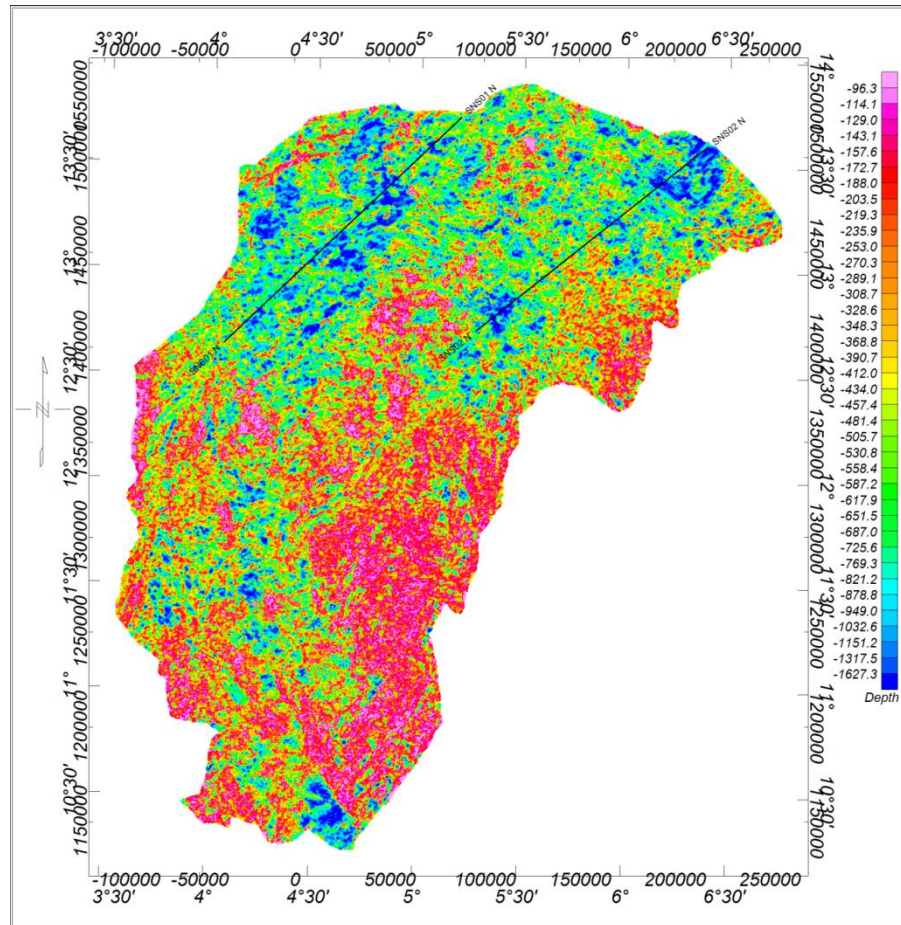
Figure 3. SPI map with profile lines across the two sub-basins (Units: Depth in metre)
