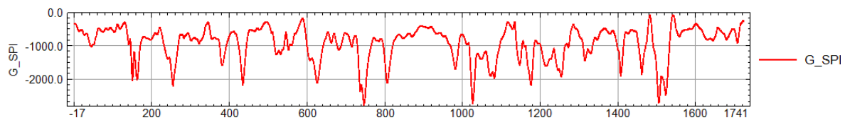
Figure 4a. Profile across Lema- Kalmalo Sub-basin
